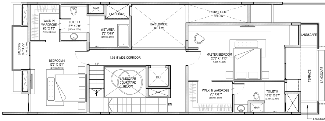
SECOND FLOOR
