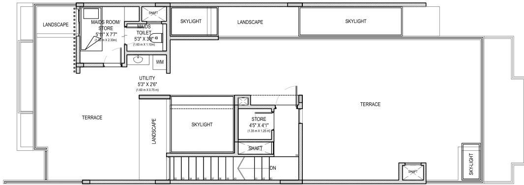
TERRACE FLOOR
